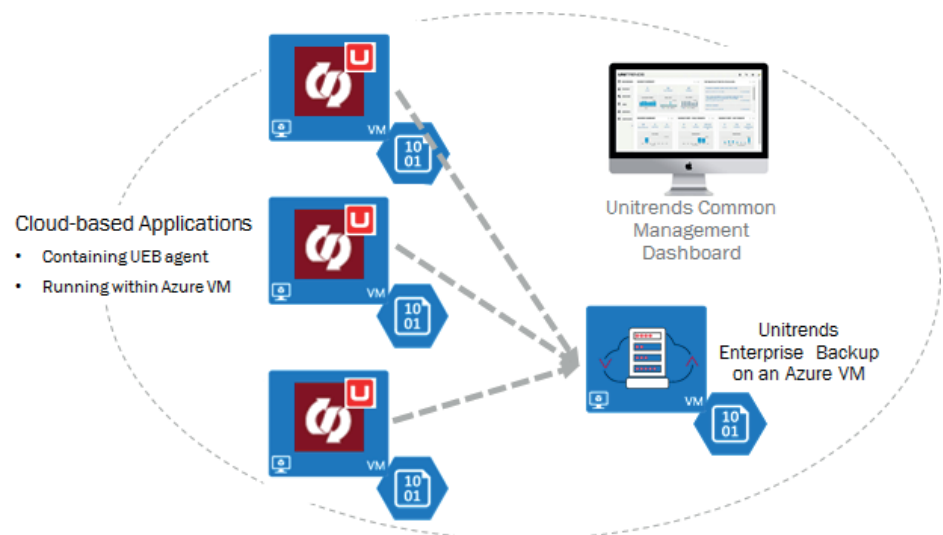
Protection for data in the cloud with Unitrends Enterprise Backup
